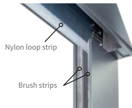
Brush strips and nylon loop strips help keep draughts at bay at the top and sides of the door.
